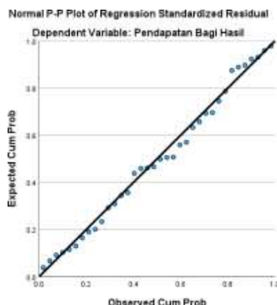
Figure 2. Results of the P-P Plot Normality Test
