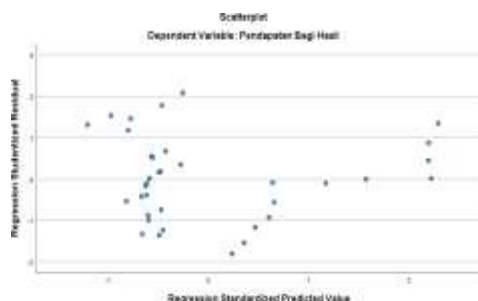
figure 3. Result Heteroskedastisitas Scatter Plot test
